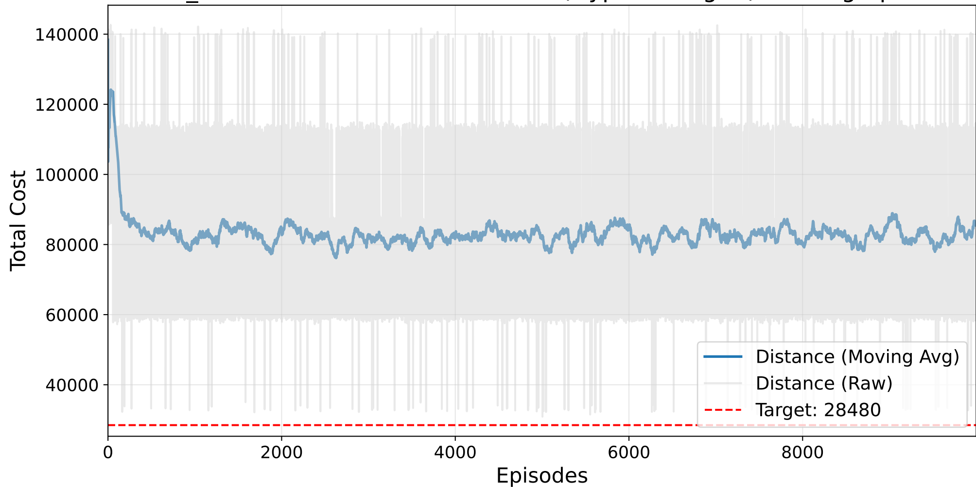
Final NO_BAYESIAN Masked AutoRL-SOP (HyperTuningSK) Training - p43.2.sop
